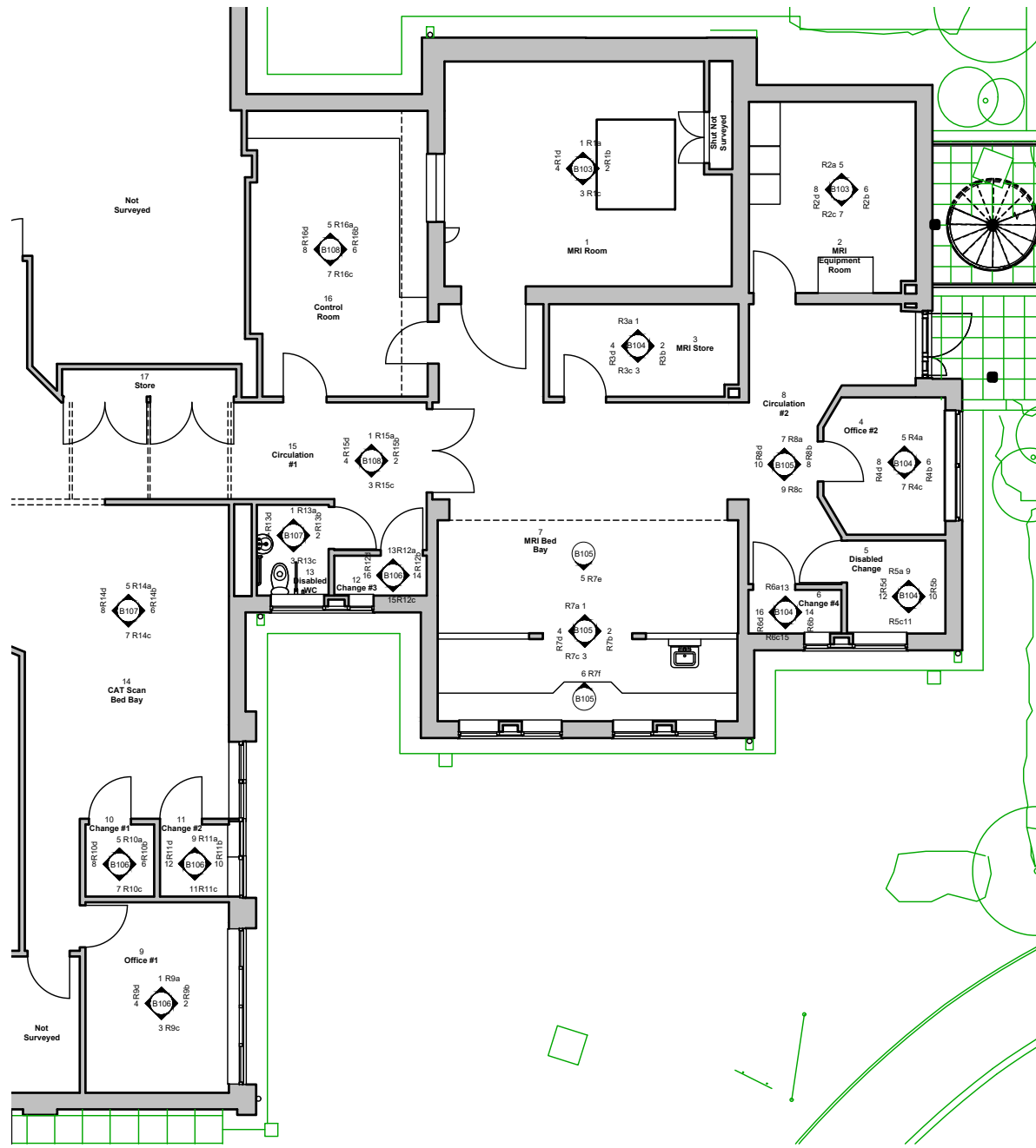
1 00-GF - Int elevation location key plan 1 : 50
